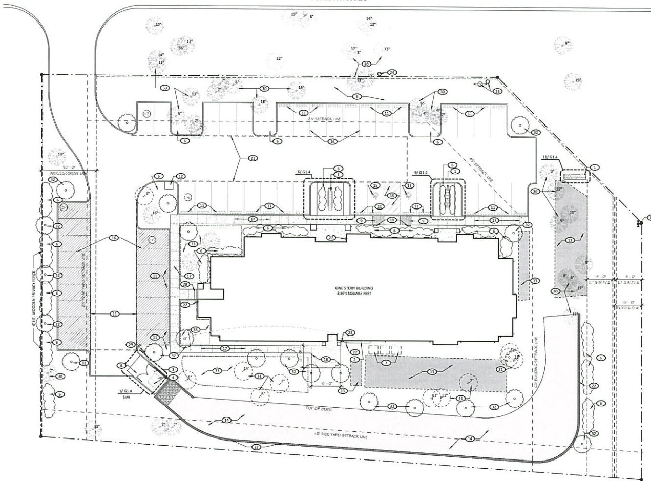
1 SITE PLAN SCALE: 1/16" = 1'-0"
